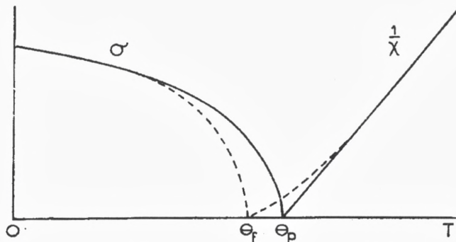
Figure 7. An early representation after Néel in Le Magnetisme (1940) of “effect des fluctuations du champ moleculaire...” At T \rightarrow T_c (= \Theta_f) the critical effects give \chi^{-1} \sim (T - T_c)^\gamma with \gamma > \gamma_0 = 1 and \sigma \sim (T_c - T)^\beta with \beta < \beta_0 = 1/2 where \beta_0, \gamma_0 are the mean field values.
