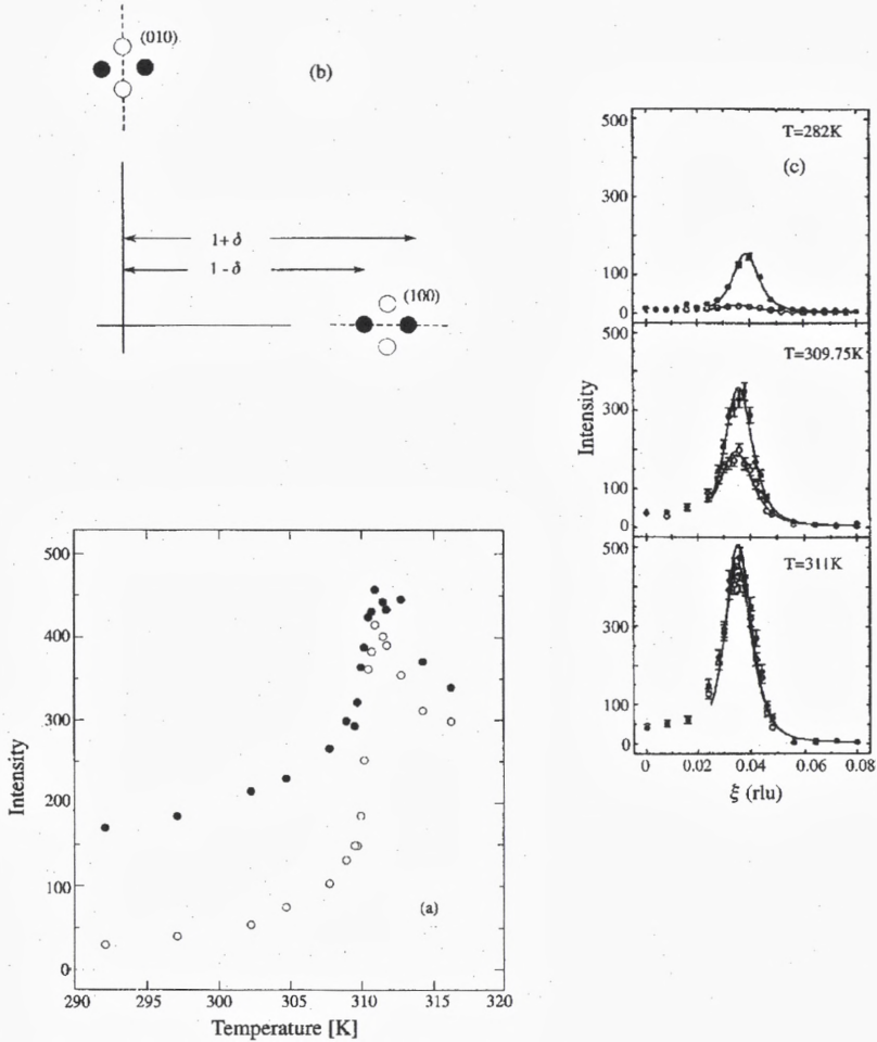
Figure 11. Silent satellites: (a) temperature dependence of the peak intensity for longitudinal scans at constant energy, E = 0.5 meV, for single- Q Cr: ● corresponds to the q -scan ——— in inset (b); ○ corresponds to the q -scan - - - in inset (b). Inset (c) shows the data for the complete q -scan close to the Néel temperature, T_N = 310.3 K, and at a temperature 28 K below T_N (after Sternlieb et al., 1995).
