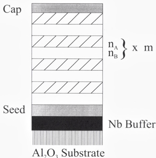
Figure 1. A schematic of the structure of a rare earth superlattice. For all of the superlattices of interest here the growth direction is parallel to the c axis of the rare earth metal. Each superlattice unit cell is made up from n_A atomic planes of element A and n_B planes of element B , with the unit cell repeated m times, so that the complete superlattice can be designated as (A_{n_A}/B_{n_B})_m . The seed layer is normally one of the non-magnetic elements Y, Lu or Sc.
