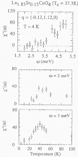
Figure 4. \chi''(q = Q_\delta, \omega) is plotted as the function of transfer energy, \omega at T = 4 K (top). Temperature dependence for \omega = 2 meV (middle), and 3 meV (bottom) are also shown (Yamada et al., 1995).
