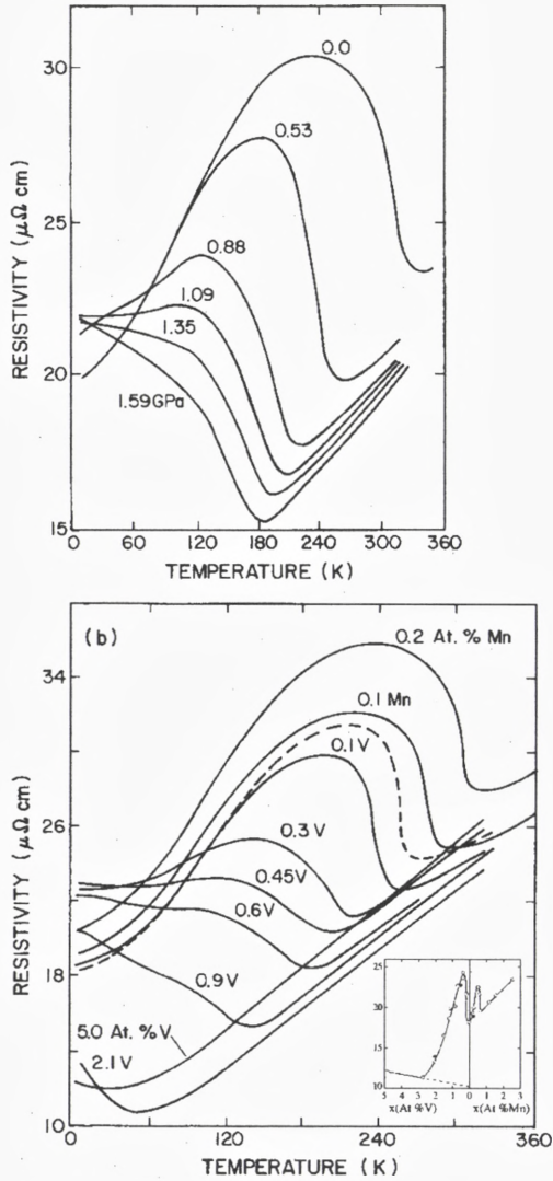
Figure 6. (a) Pressure dependence of the resistivity of Cr+2.7 at.% Fe+0.27% Mn (from Galkin, 1989). (b) Temperature dependence of the resistivity of ternary alloys (\text{Cr}+2.7 \text{ at.\% Fe})_{1-x}(\text{V},\text{Mn})_x , with the concentrations x of V or Mn shown on the curves, the curve for undoped Cr+2.7 at.% Fe being dashed (after Galkin and Fawcett, 1993). The inset shows the residual resistivity at temperature 4.2 K as a function of alloy composition (from Galkin, 1989).
