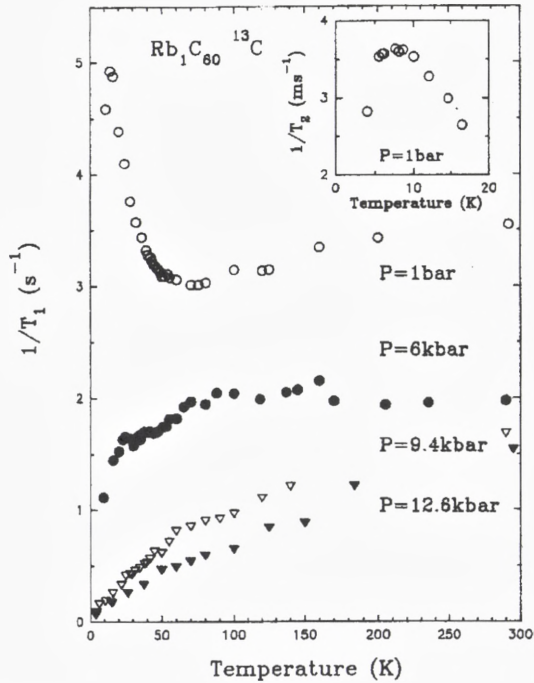
Figure 17. Temperature dependence of ^{13}C-T_1^{-1} at different pressures.
