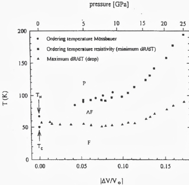
Figure 9. The ordering temperature deduced from Mössbauer spectroscopy (circles) and from resistance measurements (squares) versus volume reduction (pressure on the top scale) for NpGa 3 . The maximum of the derivative dR/dT of the low-temperature drop in resistance is also plotted (triangles). The phase diagram, P = paramagnetic, AF = antiferromagnetic, and F = ferromagnetic is proposed. (Taken from Zwirner et al., 1996)
