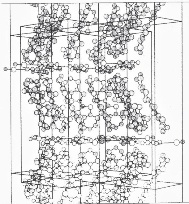
Figure 2. Transverse view of the 2D organic superconductor \kappa -(ET) 2 Cu[N(CN) 2 ]Br.
