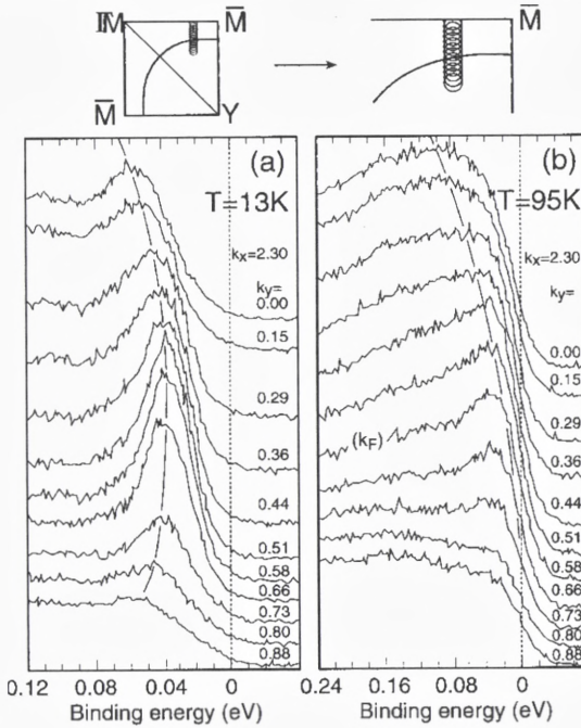
Figure 8. Photoelectron spectra from Bi2212 above and below T_c . The solid curve is a guide to the eye. In the normal state, the curve approaches close to the Fermi level while in the superconducting state, it approaches, then retreats. The wave vectors are in units of (1/a) . (Campuzano et al., 1996).
